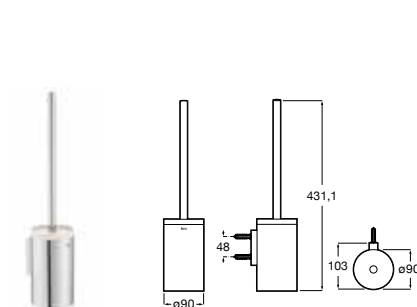
Escobillero pared
